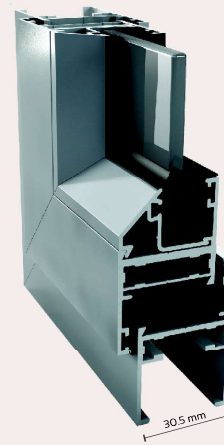
A 3D presentation of the Crealco Swift 30.5 cross-section
